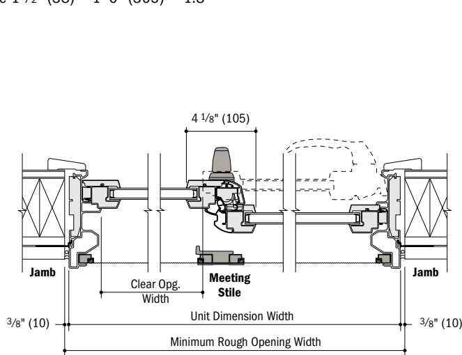
Horizontal Section
