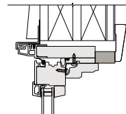
Head - Curved Arch Casement, Unequal Leg Arch Casement, Springline™ and Springline Flanker Casements
