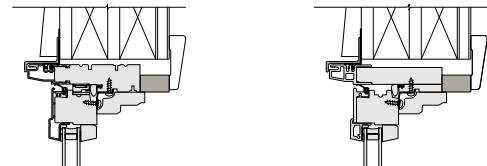
Head - Lineal Trapezoid Casement
