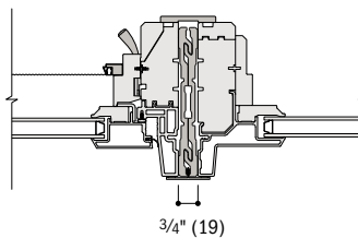
Casement to Picture Casement Lock Jamb
