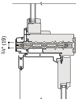
Sash-Set Specialty Over Hinged Inswing Patio Door Fiberglass – 6 9/16" (167) Base Jamb Depth
