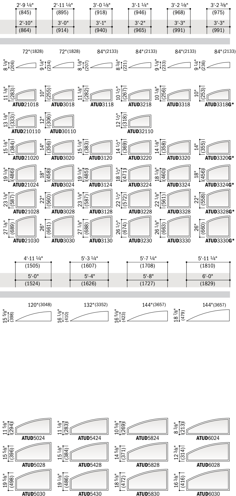
Direct-Set Unequal Leg Arch
