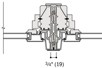
Casement to Casement Stationary Jamb to Stationary Jamb
