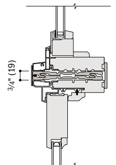
Sash-Set Specialty Over Patio Door Sidelight Fiberglass
