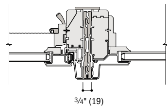
Awning to Picture
