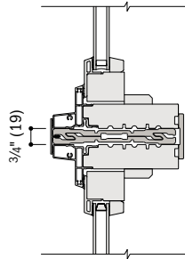
Sash-Set Specialty Over Sash-Set Specialty Fiberglass
