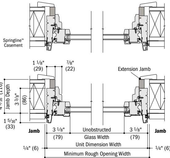
Horizontal Section Casement, Trapezoid Casement, Arch Casement and Unequal Leg Arch Casement
