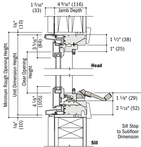
Vertical Section
