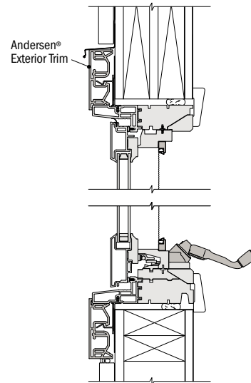
Vertical Section
