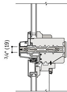
Direct-Set Specialty Over Casement/Awning Fiberglass
