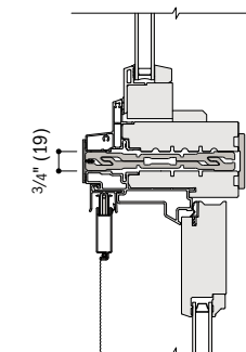
Sash-Set Specialty Over Hinged Inswing Patio Door Fiberglass – 4 9/16" (116) Base Jamb Depth
