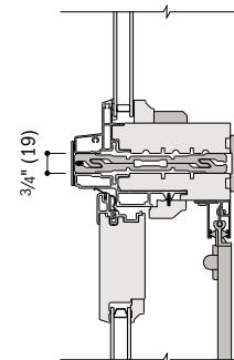
Direct-Set Specialty Over Hinged Outswing Patio Door Fiberglass
