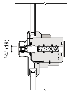
Direct-Set Specialty Over Picture Clip
