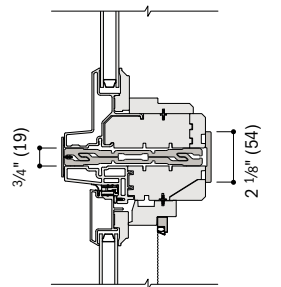
Fixed Transom Over Casement/Awning
