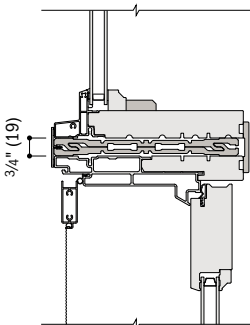
Direct-Set Specialty Over Hinged Inswing Patio Door Fiberglass – 6 9/16" (167) Base Jamb Depth
