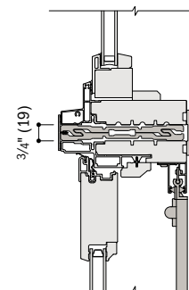
Sash-Set Specialty Over Hinged Outswing Patio Door Fiberglass
