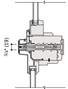
Sash-Set Specialty Over Picture Fiberglass
