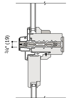
Direct-Set Specialty Over Patio Door Sidelight Fiberglass
