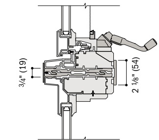
Venting Transom Over Picture
