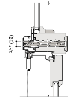
Direct-Set Specialty Over Hinged Inswing Patio Door Fiberglass – 4 9/16" (116) Base Jamb Depth
