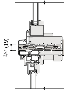
Sash-Set Specialty Over Double-Hung Fiberglass
