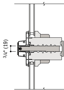
Direct-Set Specialty Over Direct-Set Specialty LVL (Factory-Joined)
