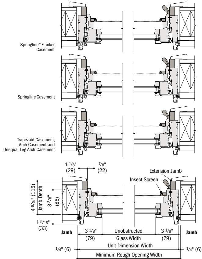
Horizontal Section Casement
