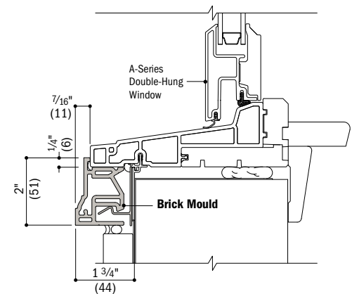
Vertical Section
