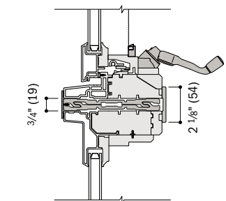
Venting Transom Over Fixed Transom
