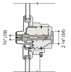
Fixed Transom Over Venting Transom
